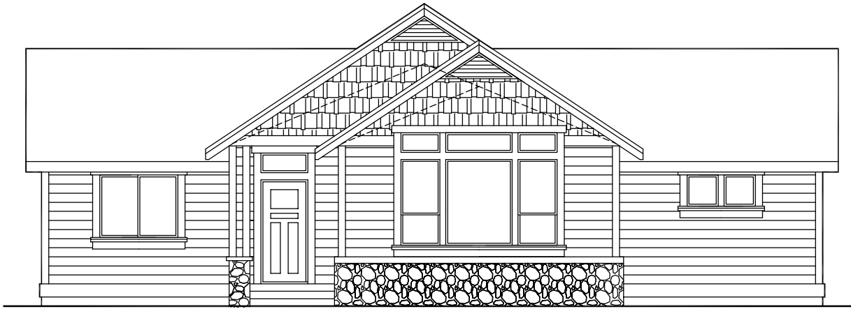
FRONT ELEVATION
