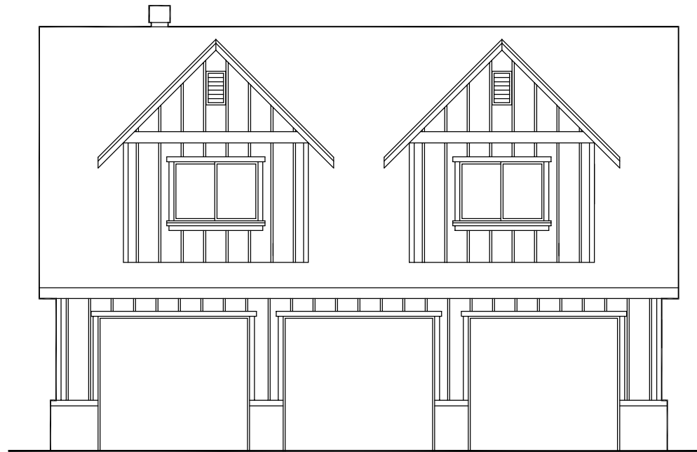
FRONT ELEVATION
