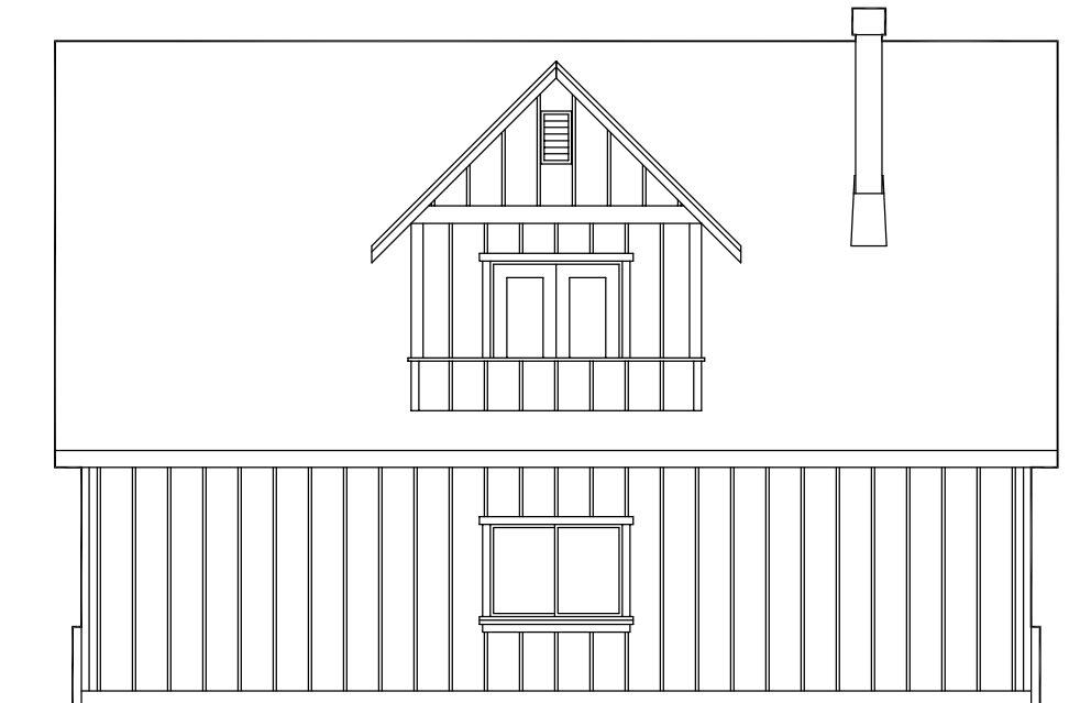
REAR ELEVATION
